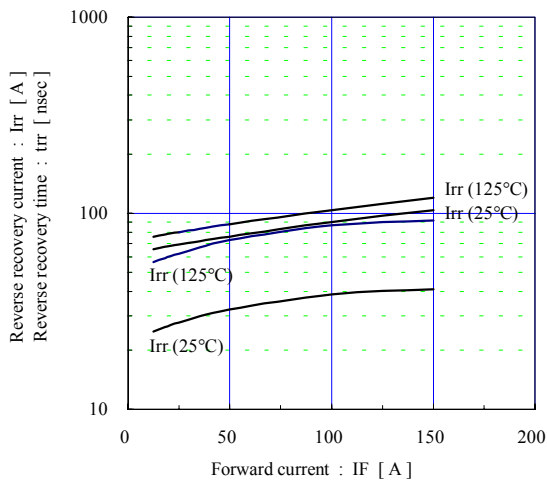
Reverse recovery characteristics (typ.) Vcc=300V, VGE=±15V, Rg=33Ω
