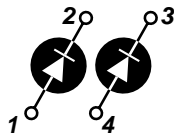
Parallel APT2X61D60J
