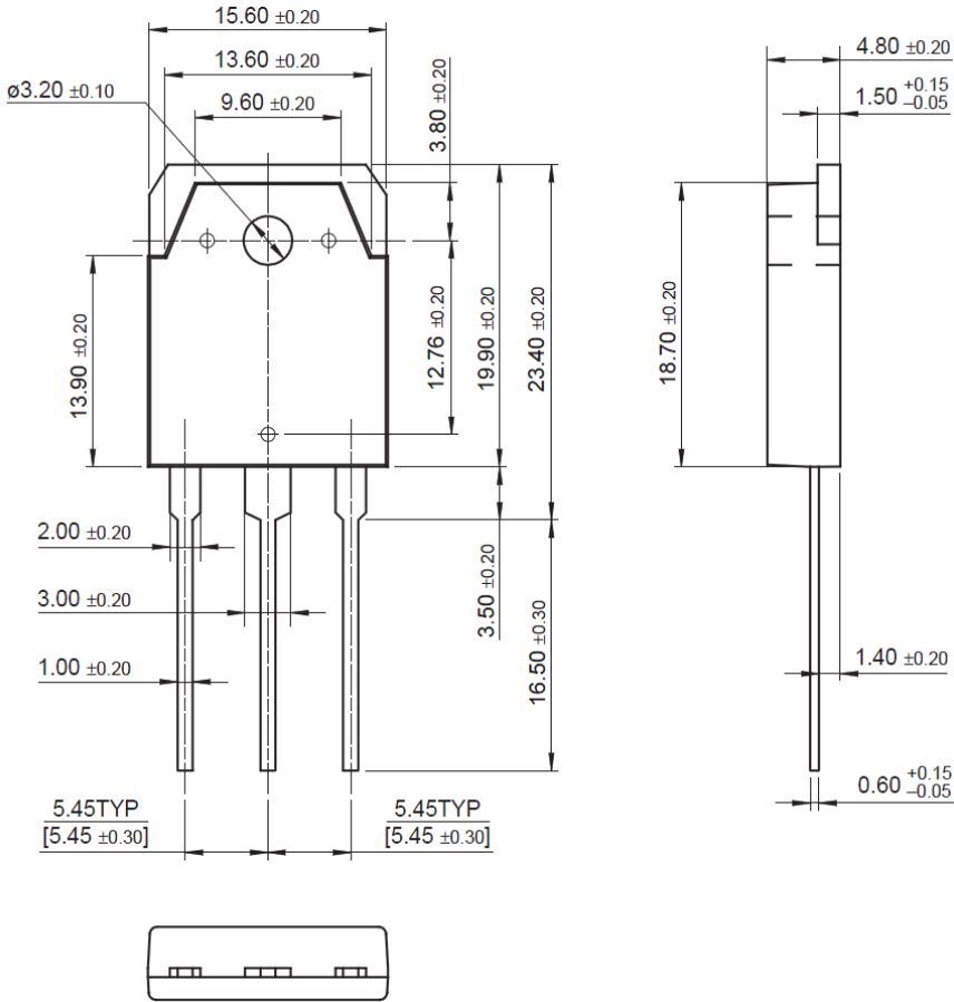
Dimensions in Millimeters Fig8. Package Outline
