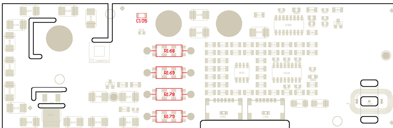
Fig. 2: Assembly drawing of 1SP0635D2Sx with highlighted gate resistors
